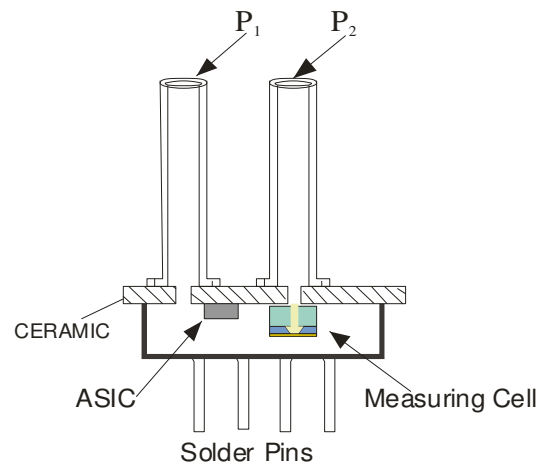
Figure 1: Dual-in-Line Pressure sensors from the AMS 5812, AMS 5612, AMS 5915 and AMS 5105 series, side view and schematic profile (Dimension: ceramic substrate 15.2x15.2mm 2 )
