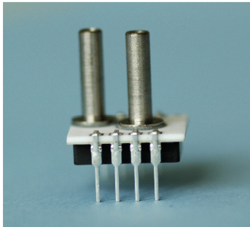
Figure 1: Dual-in-Line Pressure sensors from the AMS 5812, AMS 5612, AMS 5915 and AMS 5105 series, side view and schematic profile (Dimension: ceramic substrate 15.2x15.2mm 2 )
