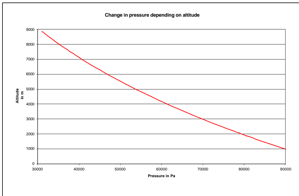
Figure 2: Change in pressure depending on altitude
