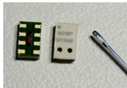
Figure 3: Pressure sensor MS5607
