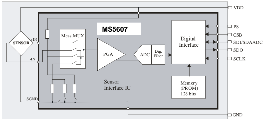
Figure 4: Principle circuitry for MS5607
