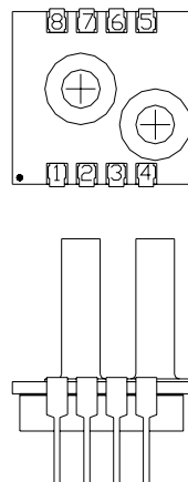
Figure 7. SM5812/SM5852 package pin-out diagram
