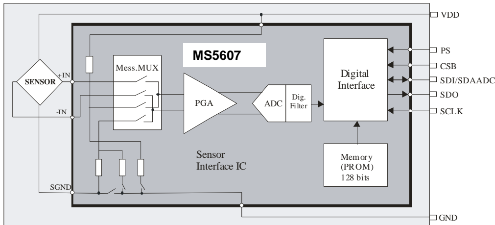
Figure 4: Principle circuitry for MS5607
