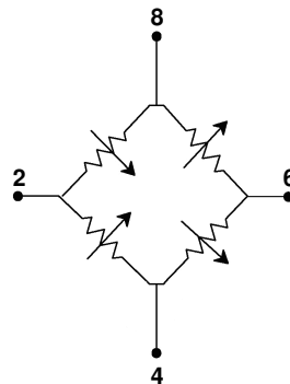
SM5420C Pin-out
